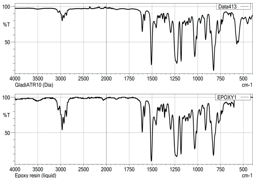
Figure 1 - IR spectrogram of ED-20 epoxy resin
