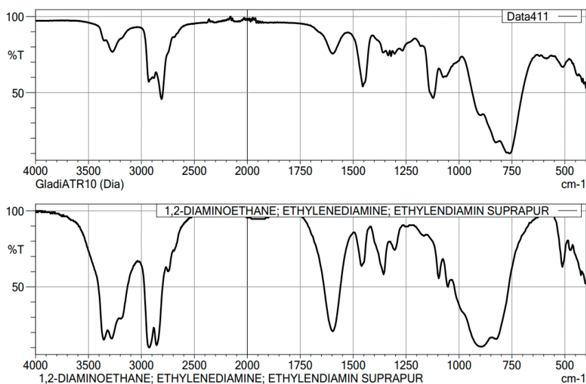
Figure 2 - IR spectrogram of PEPA hardener
