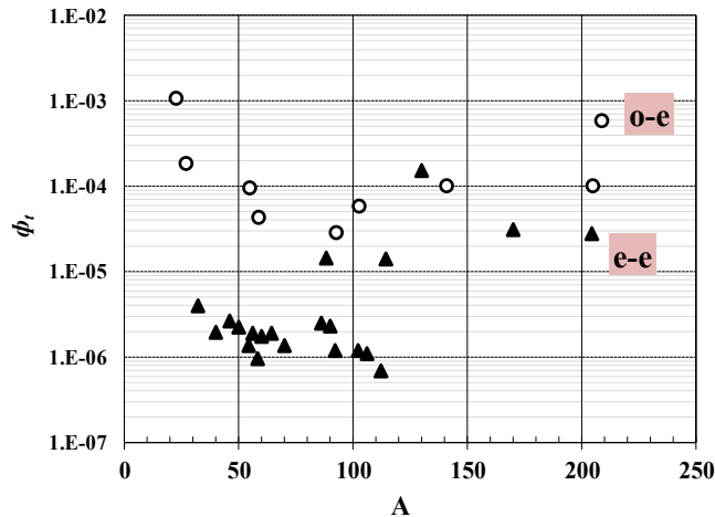
Figure 2 - The dependence of the triton clustering factors on the mass number of target nuclei: (o-odd-even and ▲-even-even nuclei)
