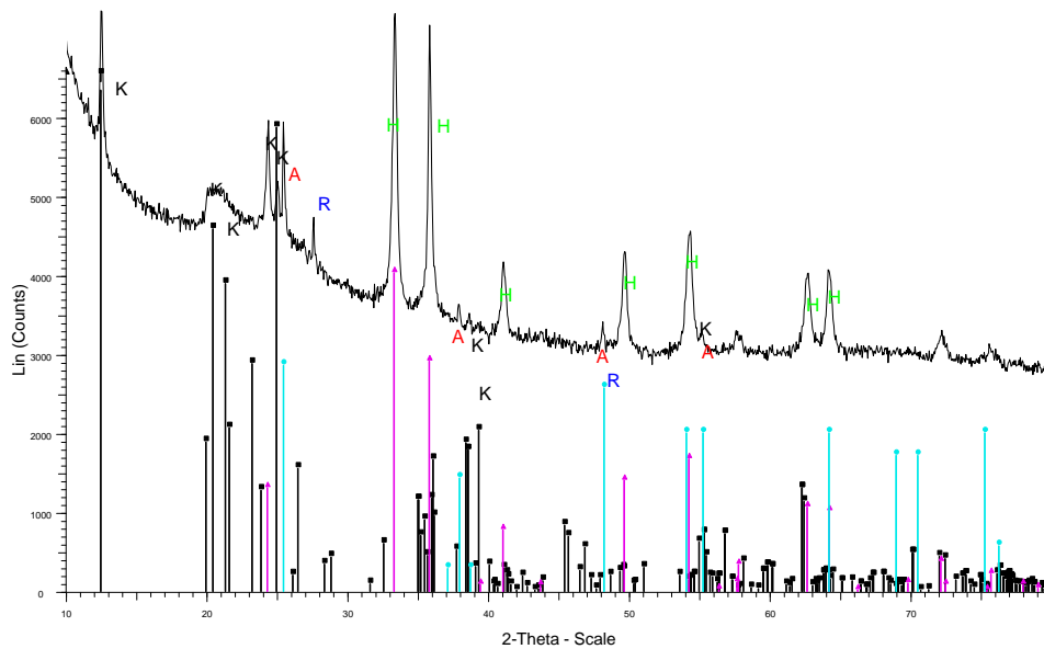
Figure 1 - Diffraction pattern of a sample of the original natural clay: K-kaolinite, A-anatase, R-rutile, H-hematite
