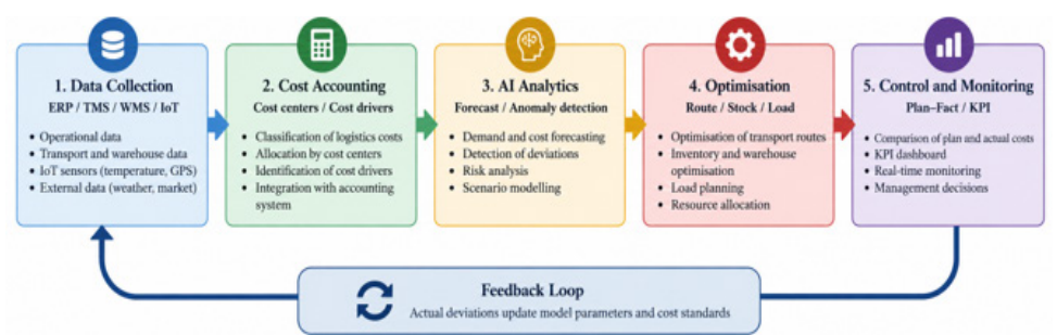
Figure 2 — Architecture of AI-enabled control of logistics costs Note: developed by the authors.
